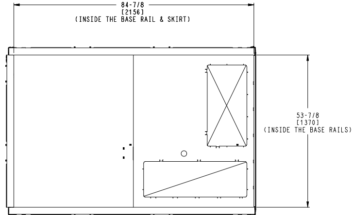
INSIDE BASERAIL DIMENSIONS BOTTOM
